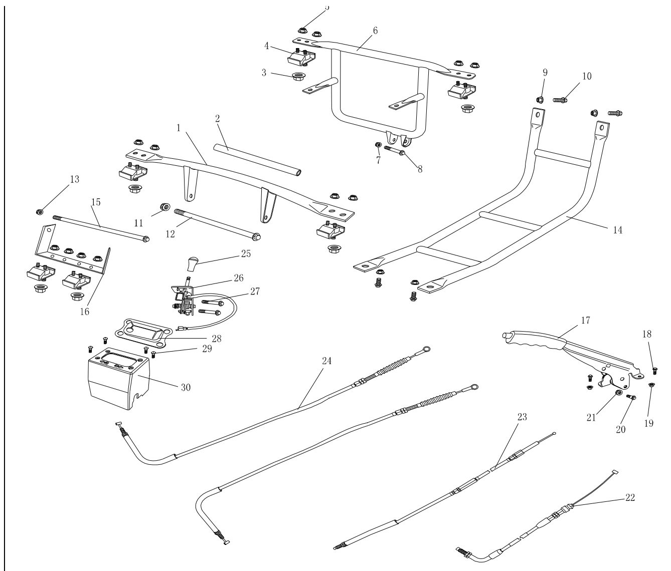
F-6 后悬挂系统发动机保护杠 ---REAR HANG/ENGINE PROTECTION STICK.
