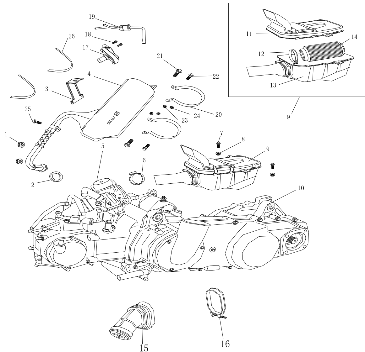
F-10 发动机、消音器、空滤器、化油器---ENGINE/MUFFLER/AIR CLEANER/CARBURETOR
